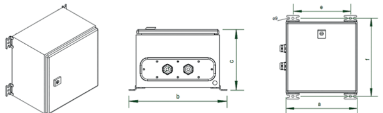
IP54 dV/dt Filter - Outlines
