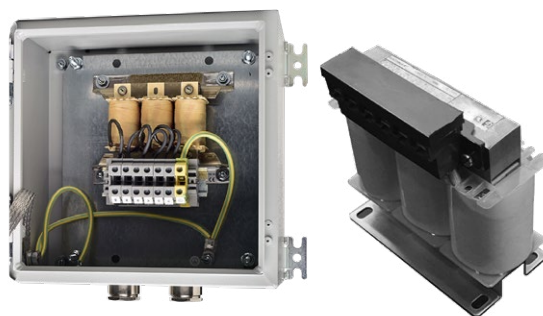
dv/dt output filter
